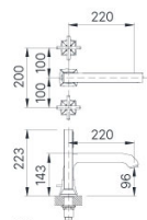
BFV-8100B Giá: 11.100.000 VNĐ
