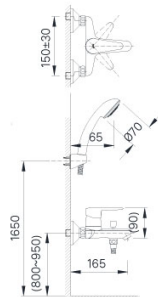
BFV-1103S-4C Giá: 1.940.000 VNĐ
